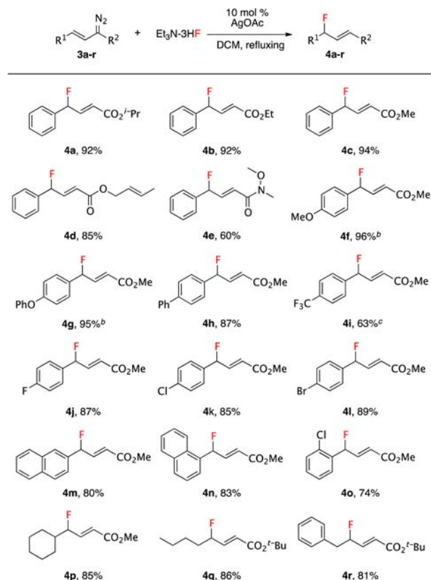
Scheme 1. Synthesis of Secondary Allylic Fluorides a
